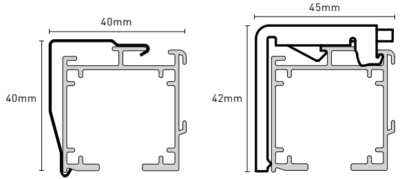
Low profile mounting clips
